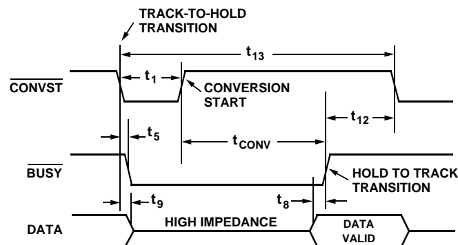
Figure 11. Conversion Start and Data Read Timing Diagram, ( \overline{CS} = \overline{RD} = 0 V)
