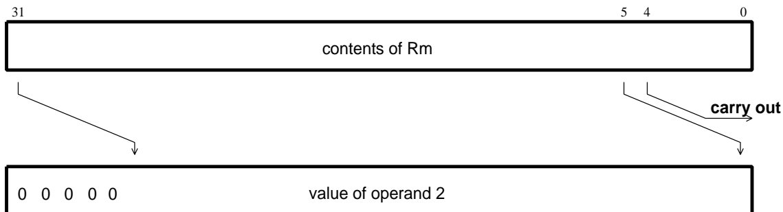
Figure 16. Logical Shift Right
