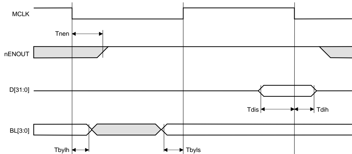
Figure 94. Bidirectional Data Read Cycle
