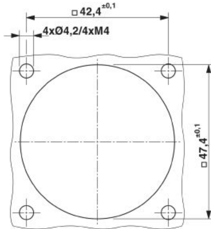
Dimensional drawing
