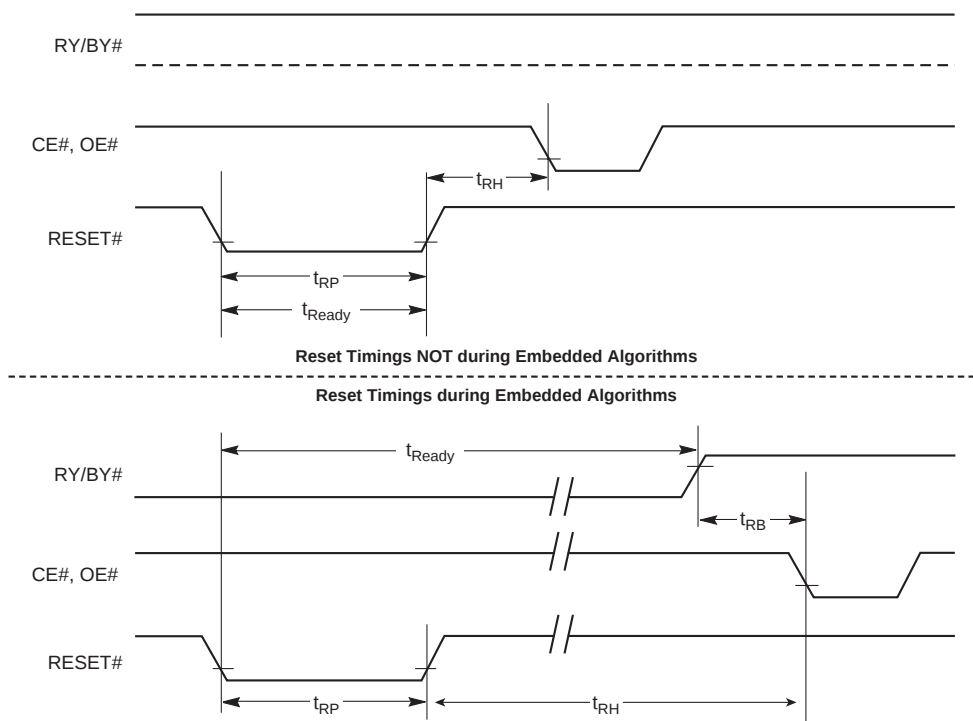
Figure 15.3 Reset Timings
