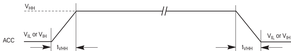
Figure 15.5 Accelerated Program Timing Diagram
