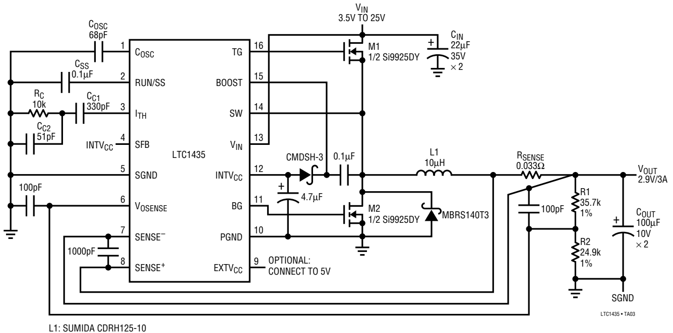
Low Dropout 2.9V/3A Converter
