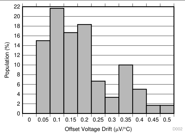
Figure 7-40. Offset Voltage Drift Distribution
