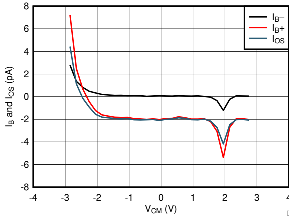
Figure 7-7. I_B and I_{OS} vs Common-Mode Voltage
