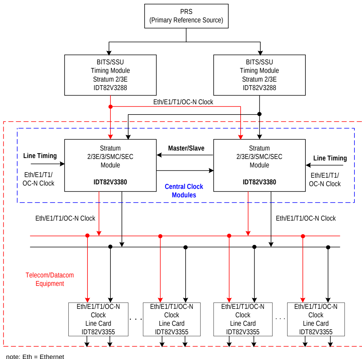
Figure 15. Typical Application
