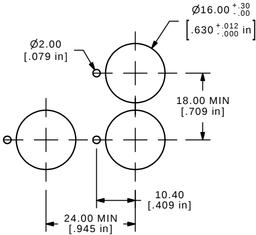
PANEL MOUNTING
