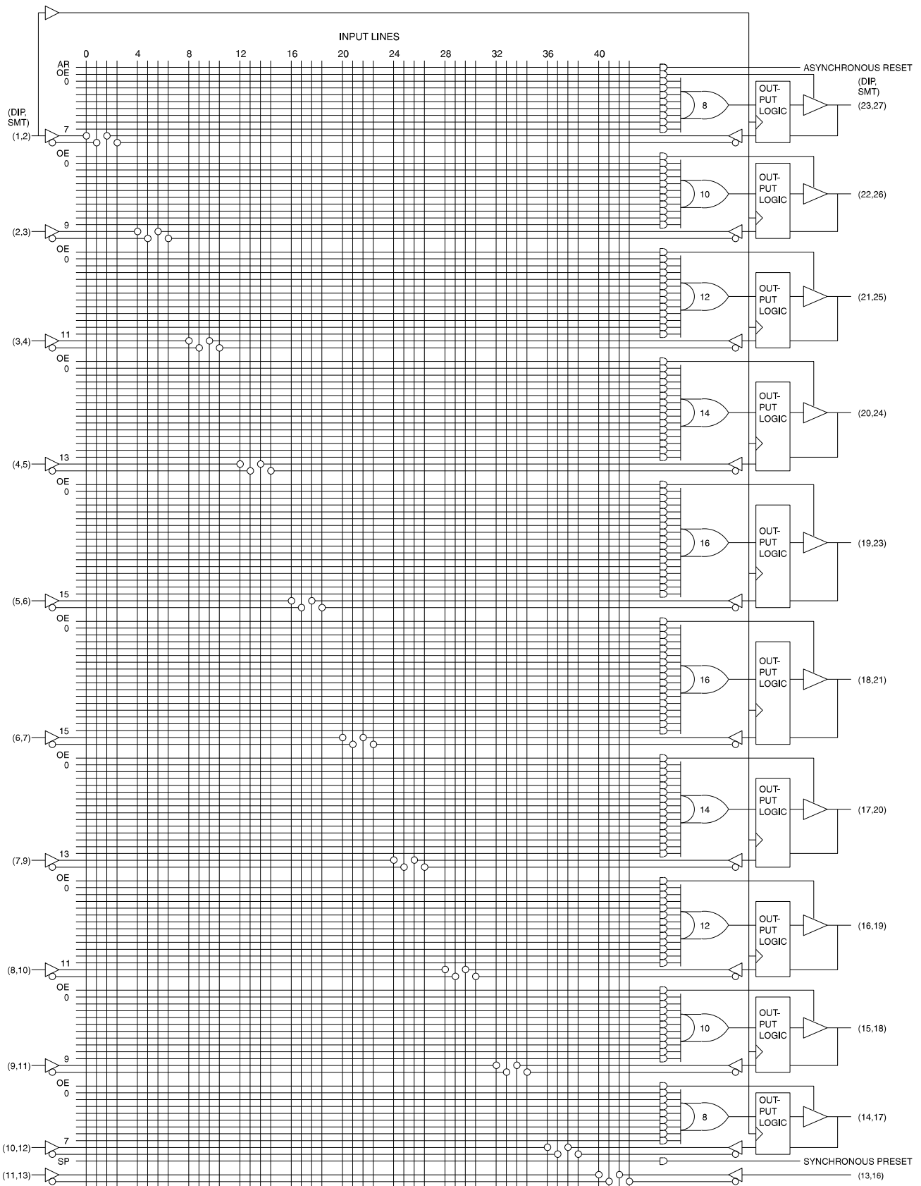
Functional Logic Diagram AT22V10/L
