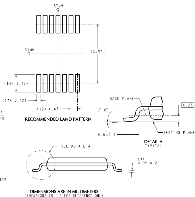
14-Pin TSSOP NS Package Number MTC14
