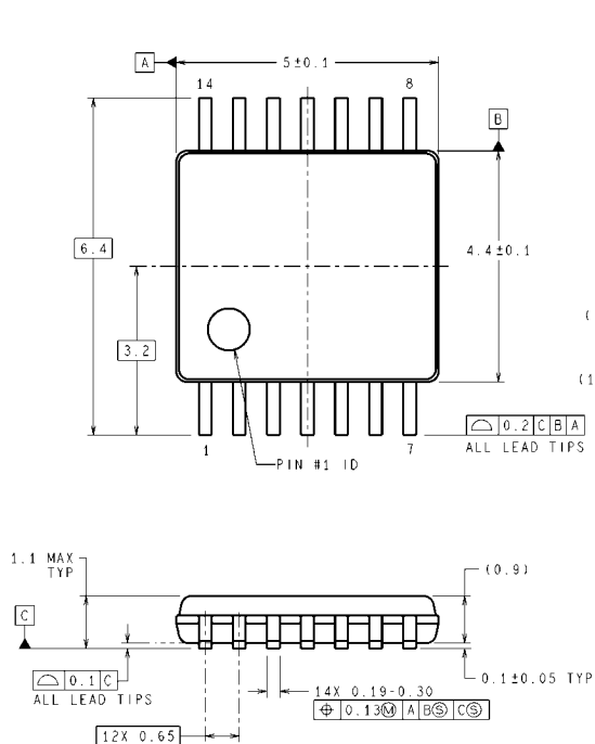
14-Pin TSSOP NS Package Number MTC14
