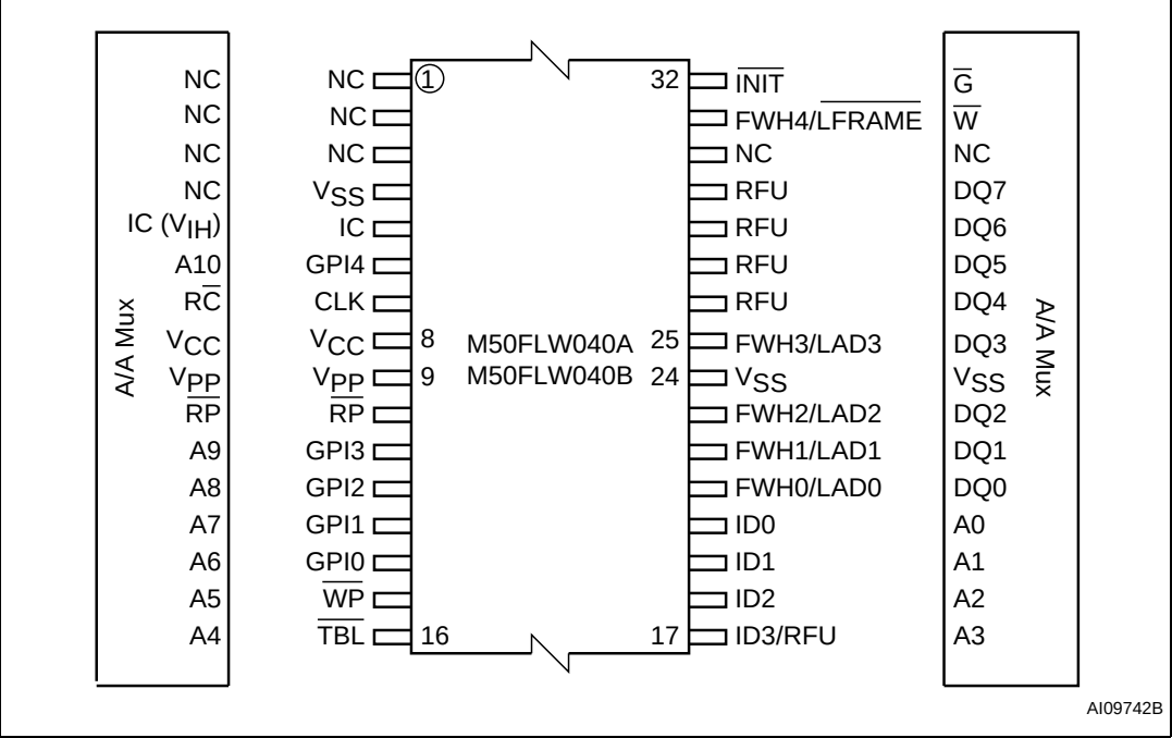
Figure 4. TSOP32 connections
