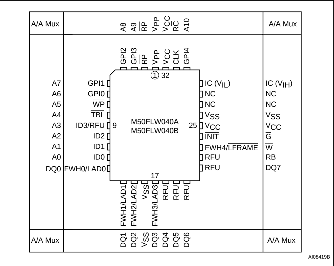
Figure 3. PLCC connections
