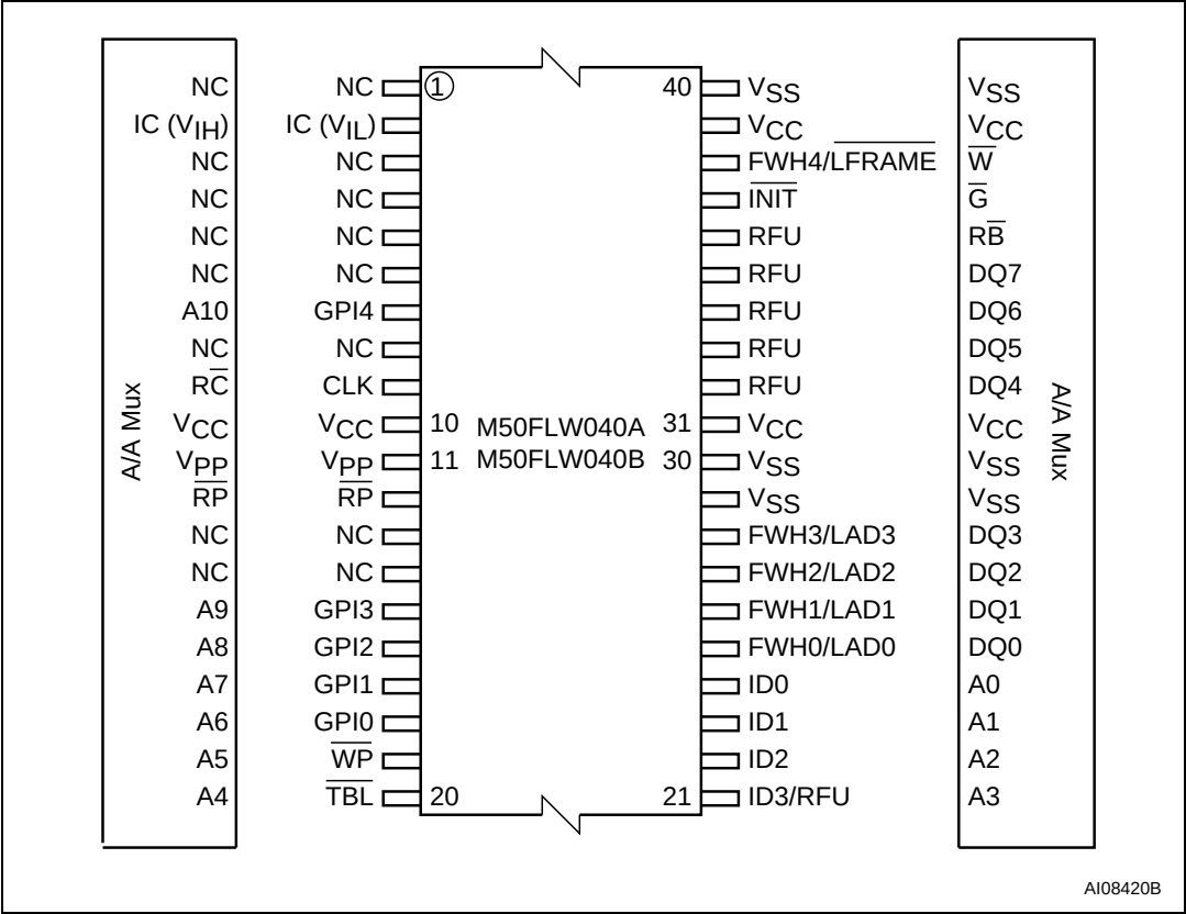
Figure 5. TSOP40 connections
