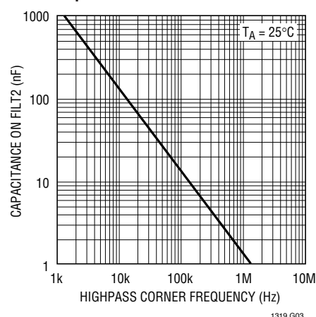
Gain Stage Highpass vs Capacitance on FILT2 or FILT2L
