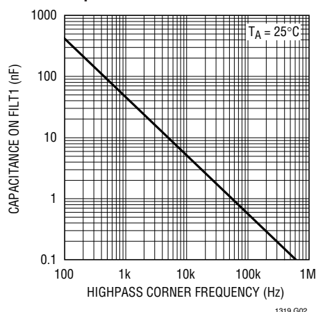
Preamp Highpass vs Capacitance on FILT1
