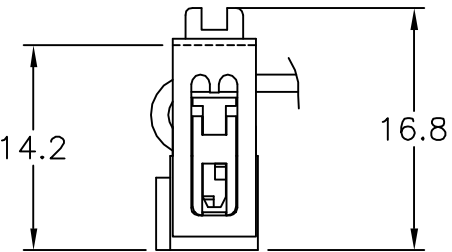
WITH STANDARD STRAIN RELIEF
