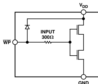
Figure 6b. Equivalent \overline{\text{WP}} Input Protection
