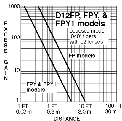
Opposed Mode—0.040 Inch Fibers and Model L2 Lenses for Extended Sensing Range
