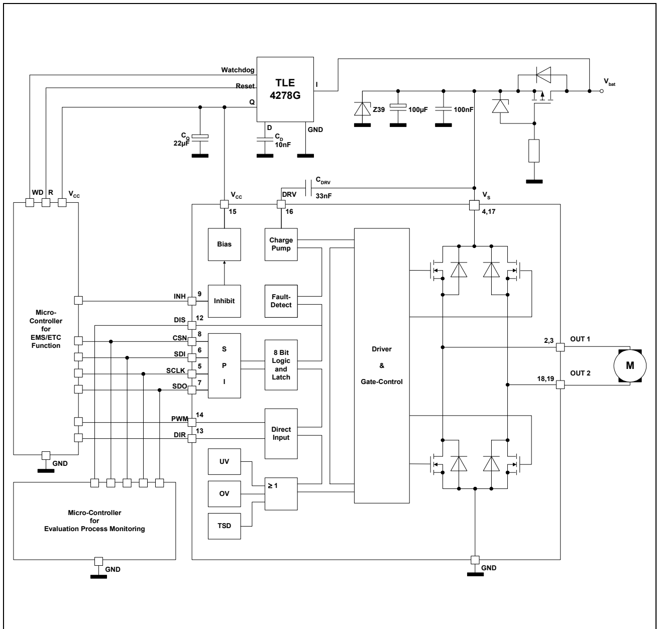
Figure 12 Application Circuit
