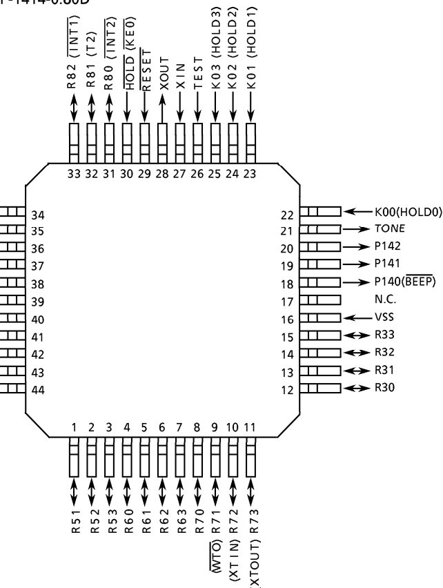
(2) QFP44-P-1414-0.80D
