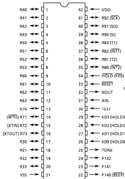
(1) SDIP42-P-600-1.78
