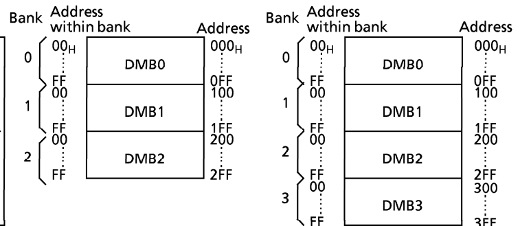
(a) 47C457
