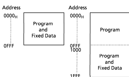
(a) 47C457
