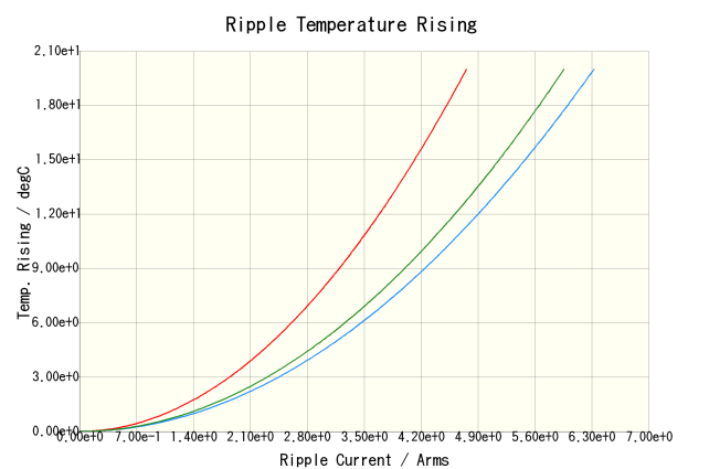
C5750X7R2A475M230KA(100kHz) C5750X7R2A475M230KA(500kHz) C5750X7R2A475M230KA(1MHz)
