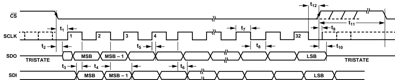
Figure 3. SPI Timing Diagram for a 32-Bit \overline{\text{CS}} Frame
