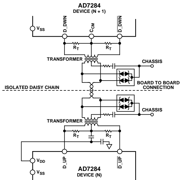
Figure 45. Transformer Configuration (Additional Circuitry Omitted for Clarity)
