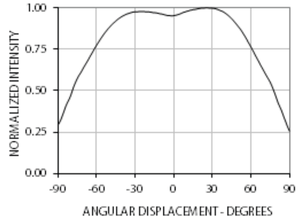
Figure 8 Radiation Pattern
