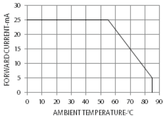
Figure 9 Derating Curve
