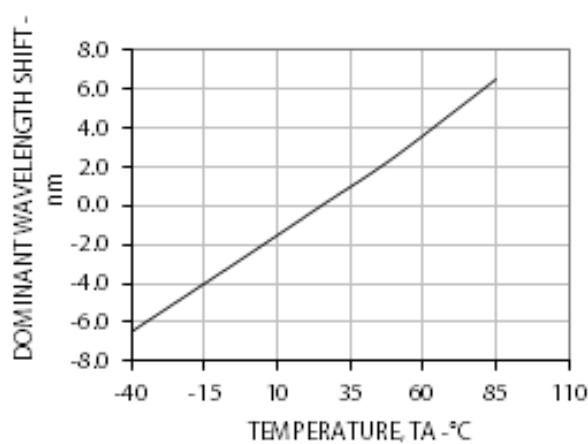
Figure 6 Dominant Wavelength Shift vs. Temperature
