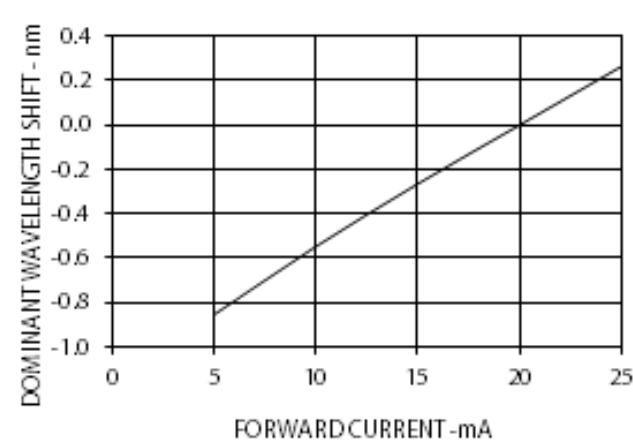
Figure 4 Dominant Wavelength Shift vs. Forward Current
