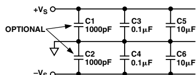
Supply Bypassing
