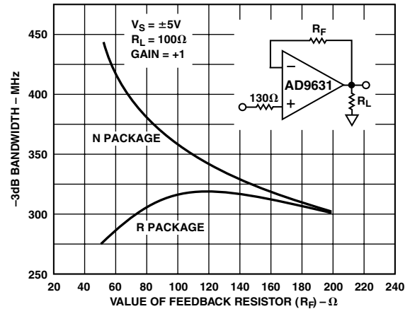
TPC 16. AD9631 Small Signal -3 dB Bandwidth vs. R_F
