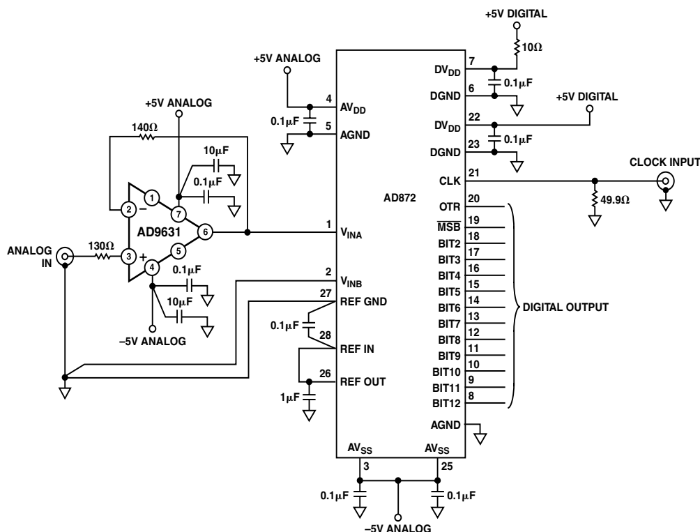
Figure 10. AD9631 Used as Driver for an AD872, a 12-Bit, 10 MSPS A/D Converter
