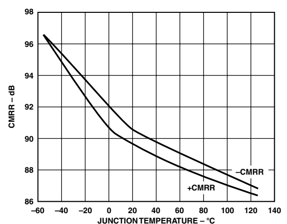
TPC 48. AD9631/AD9632 CMRR vs. Temperature
