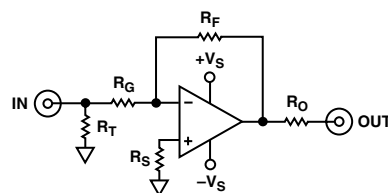
Inverting Configuration
