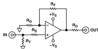
Noninverting Configuration
