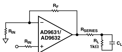
Figure 6. Driving Capacitive Loads
