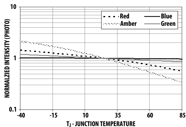
Figure 13 Relative Intensity Shift vs. Junction Temperature
