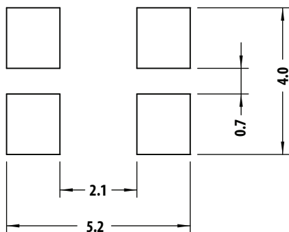
Figure 15 Recommended Soldering Land Pattern
