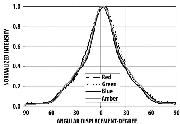
Figure 12 Radiation Pattern for Minor Axis
