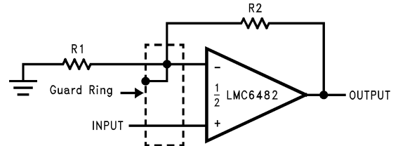
Non-Inverting Amplifier
