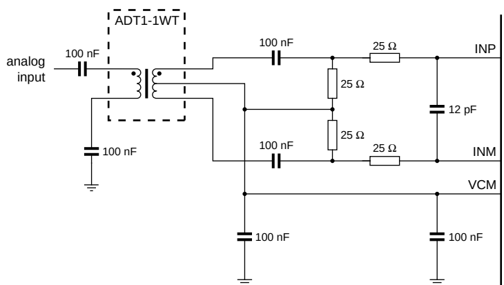
Fig 18. Single transformer configuration suitable for baseband applications
