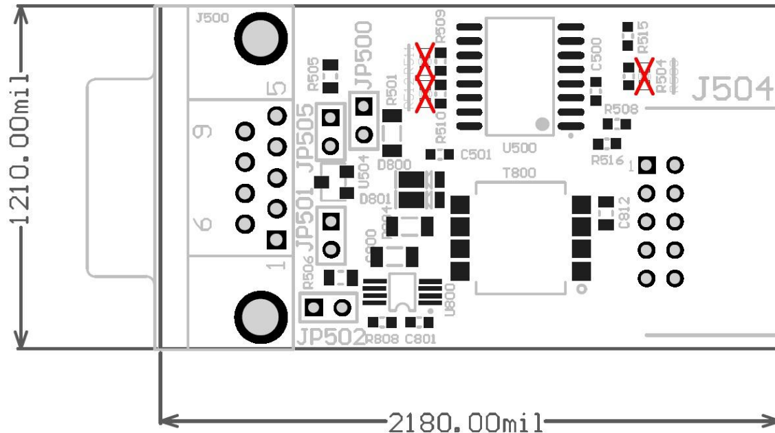
Figure 1: Dimensions 2.2" x 1.2"
