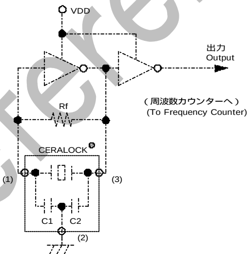
Figure 2. Test Circuit
