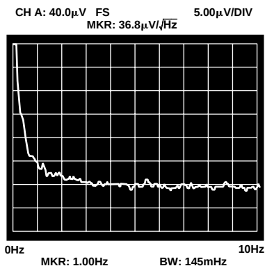
Figure 35. 1/f Noise Corner, V_S = \pm 5V , A_V = 1,000
