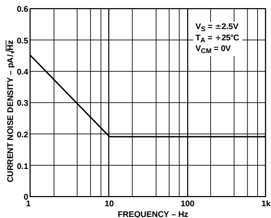
Figure 28. Input Bias Current Noise Density vs. Frequency
