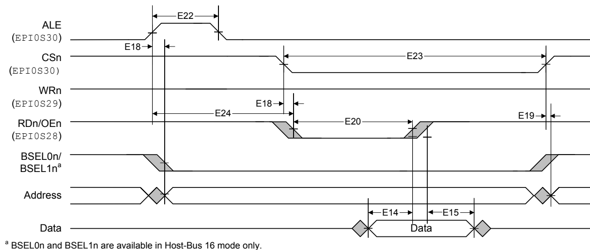
Figure 25-14. Host-Bus 8/16 Mode Read Timing
