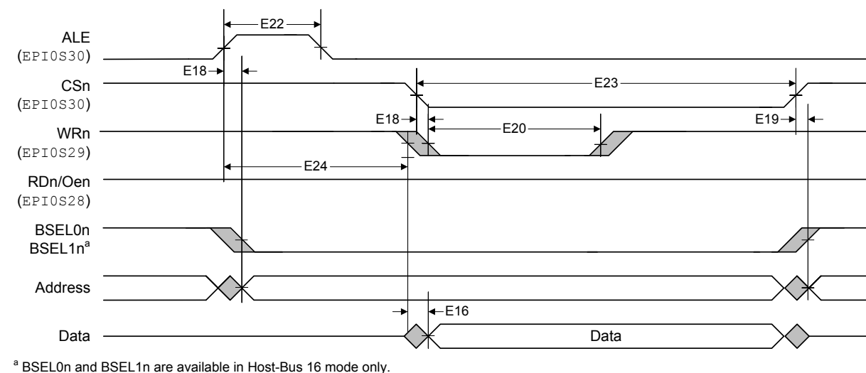
Figure 25-15. Host-Bus 8/16 Mode Write Timing
