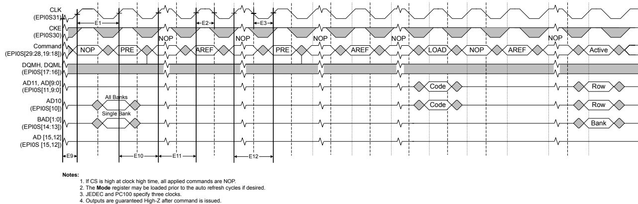
Figure 25-11. SDRAM Initialization and Load Mode Register Timing
