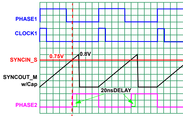
FIGURE 36. SYNCHRONIZATION WAVEFORMS
