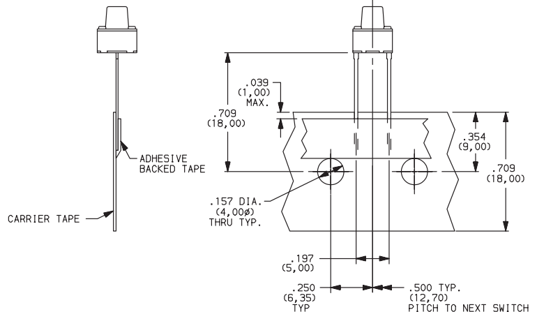
TAPE & REEL PACKAGING
