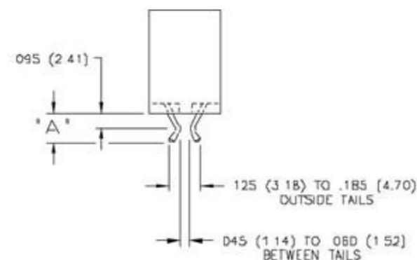
CONTACT CODE 556
