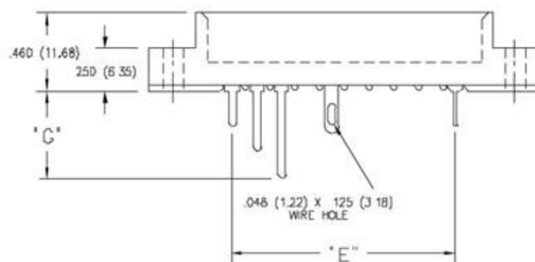
INSULATOR STYLE CODE 2
