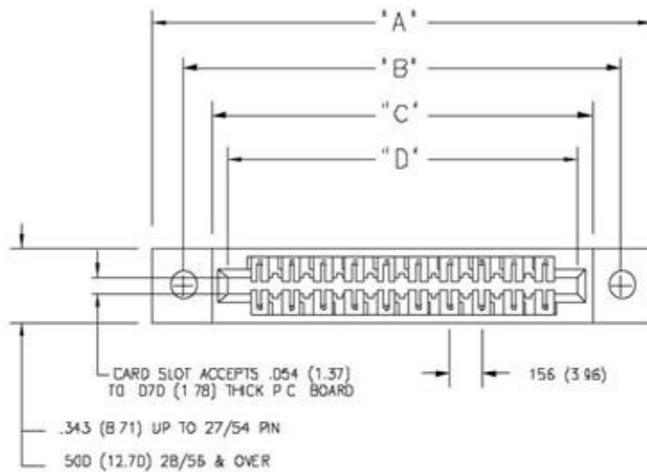
IN-CONTACT POLARIZING KEY P/N 307-240-328
