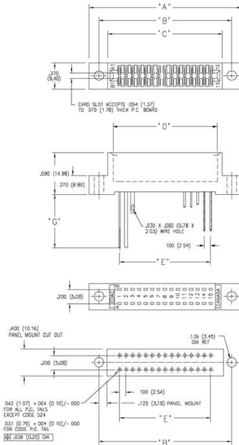
CONNECTOR MOUNTING PATTERN
