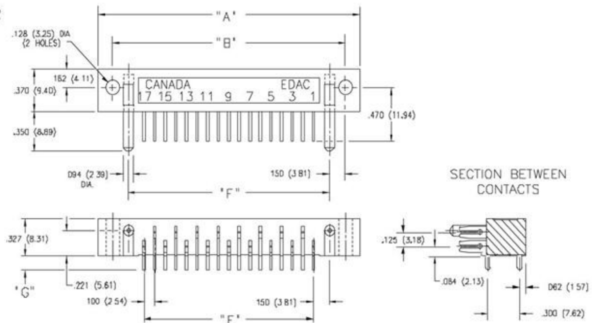
423 SERIES CONNECTOR
