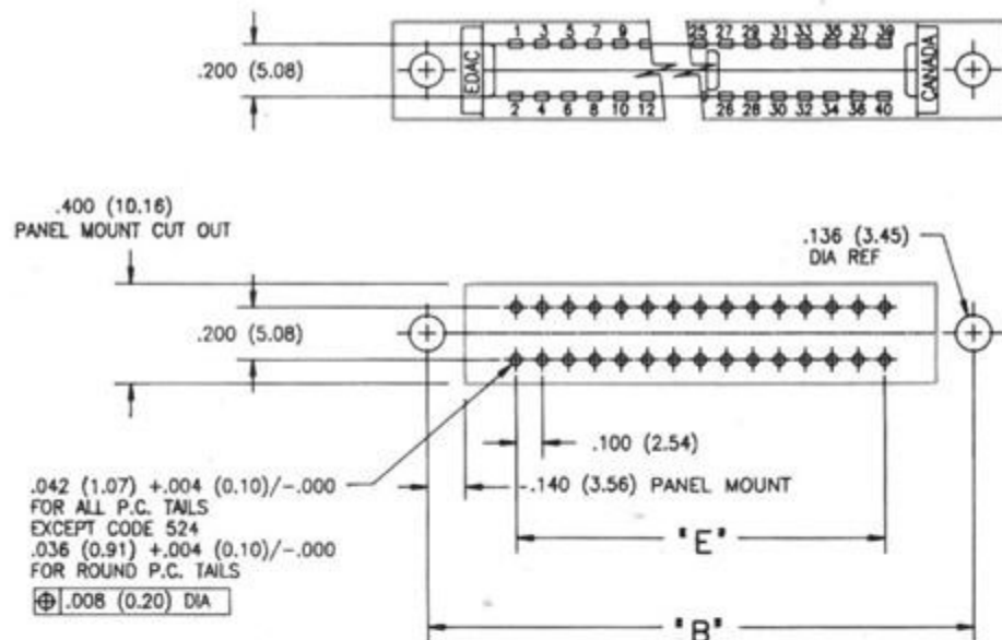
CONNECTOR MOUNTING PATTERN
