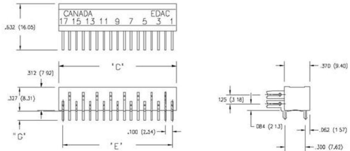
422 SERIES CONNECTOR
