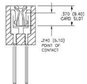
SECTION THROUGH CONTACT POSITION
