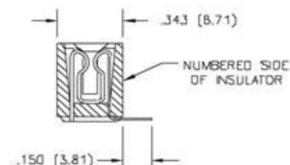
CONTACT CODE 554 BEND USES WIRE HOLE CONTACTS
