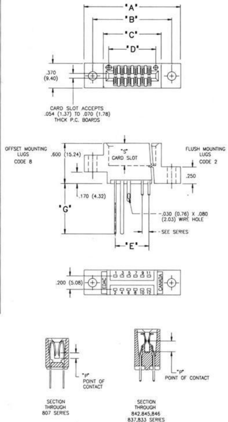
SERIES 842,845,846,837,833
