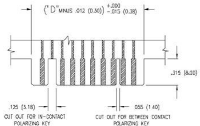
RECOMMENDED DAUGHTER BOARD
