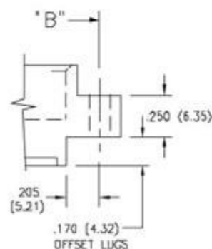
DUAL ROW
