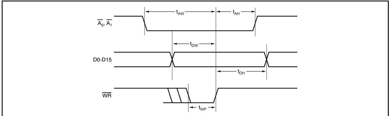
Figure 1. Timing Diagram
