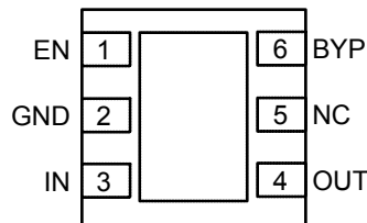
MIC5219-x.xBML 6-Pin 2mm × 2mm MLF ® (ML) (Top View)
