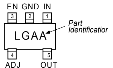
MIC5219BM5 / SOT-23-5 Adjustable Voltage (Top View)
