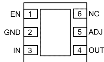
MIC5219YMT 6-Pin 2mm × 2mm Thin MLF ® (MT) (Top View)
