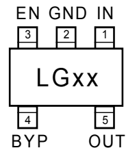
MIC5219-x.xBM5 / SOT-23-5 Fixed Voltages (Top View)
