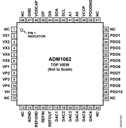
Figure 4. TQFP Pin Configuration
