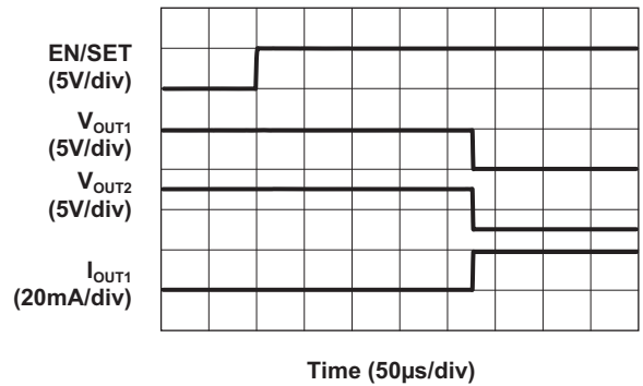
Turn-On Characteristic ( I_{OUT1} = I_{OUT2} = 20\text{mA} )
