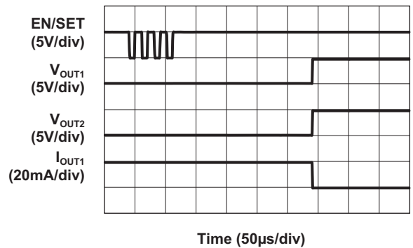
Turn-Off Characteristic ( I_{OUT1} = I_{OUT2} = 20\text{mA} )
