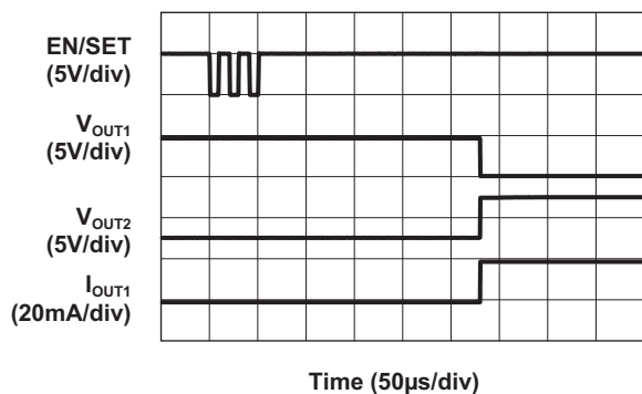
Turn-Off Transient Characteristic
