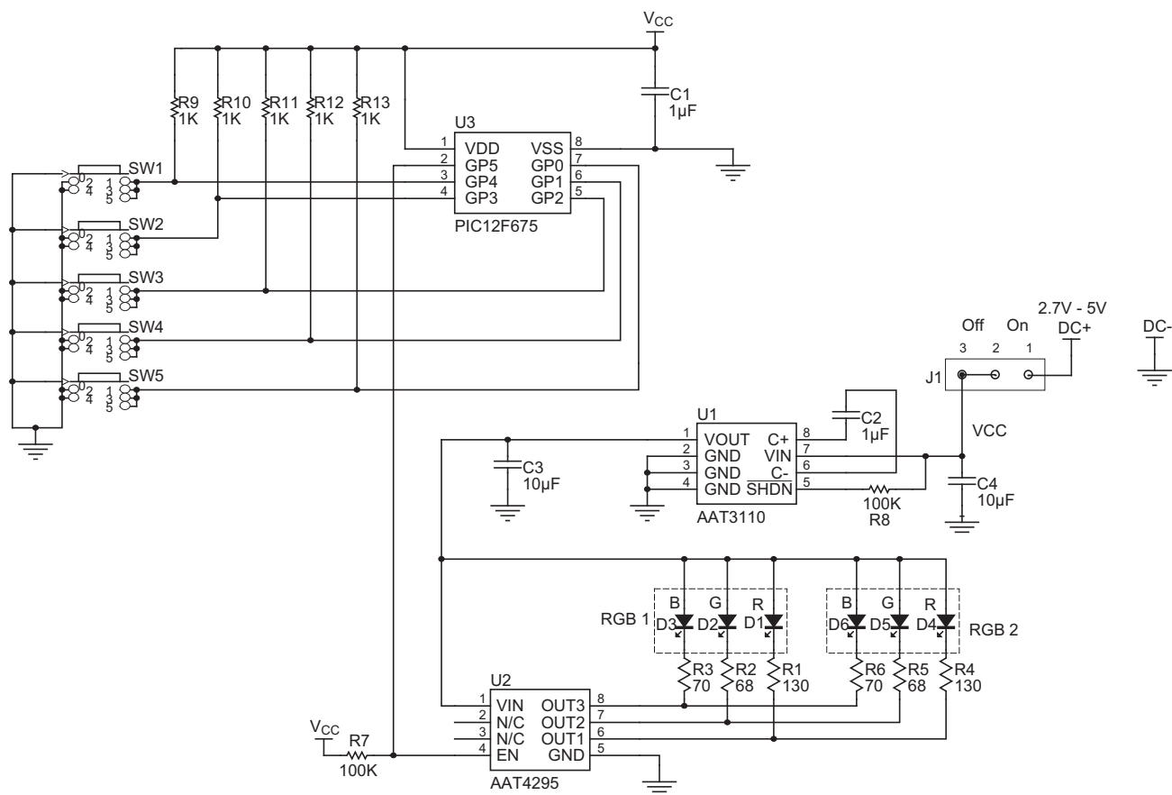
Figure 8: AAT4295 Evaluation Board Schematic.
