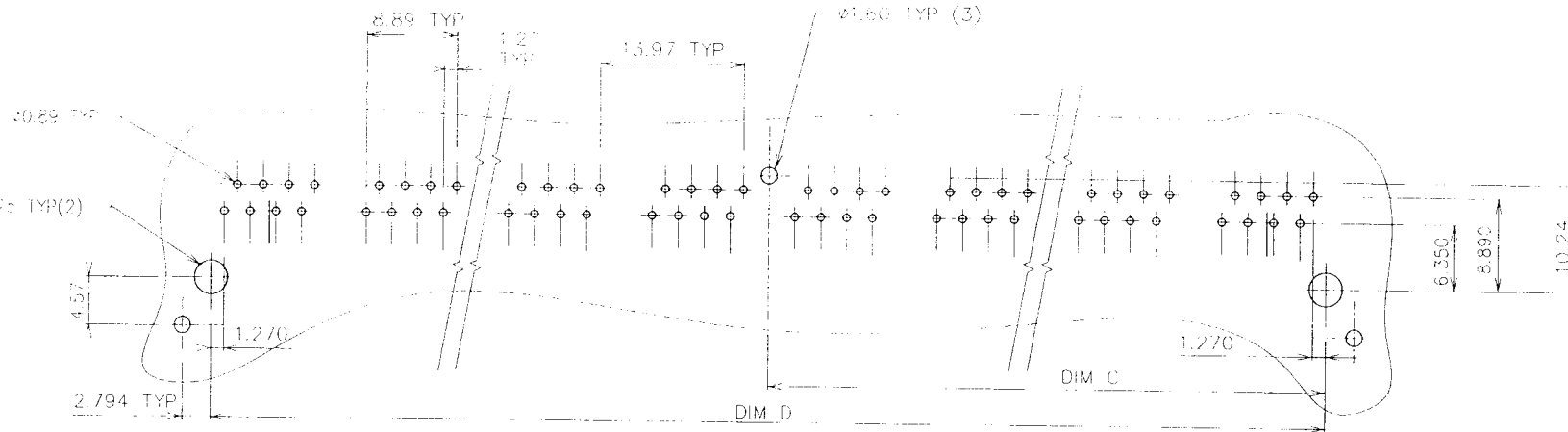
RECOMMENDED PC BOARD LAYOUT (2 THRU 12 PORTS)
