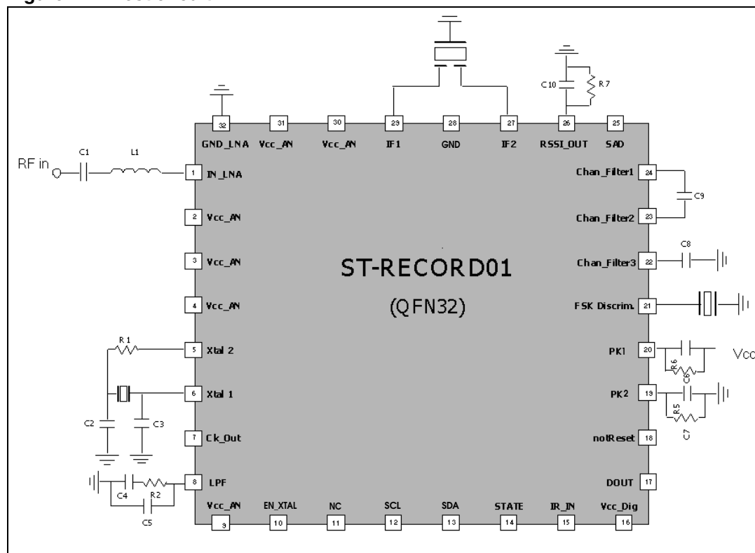
Figure 2. Test circuit
