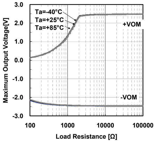
Maximum Output Voltage vs. Load Resistance V_+/V_- = \pm 2.5V , open loop
