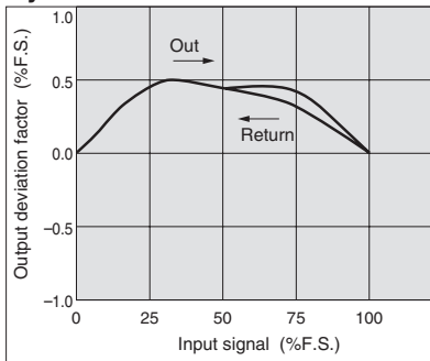
Hysteresis
