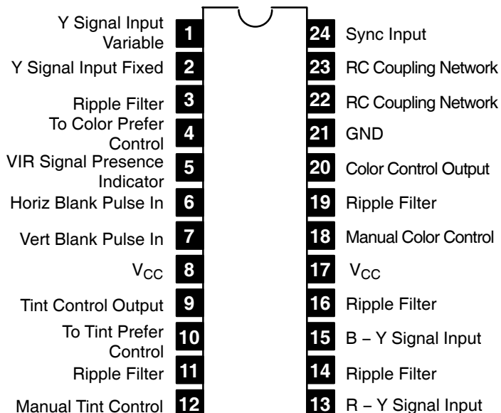
Pin Connection Diagram (Front View)
