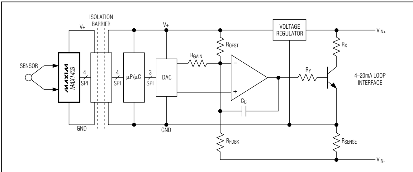
Figure 16. 4–20mA Transmitter
