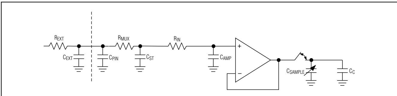
Figure 6. Analog Input, Buffered Mode (BUFF = 1)
