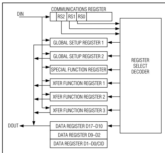
Figure 3. Register Summary
