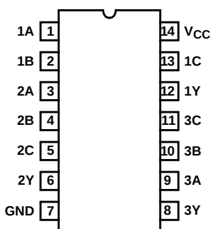
CD54HC11, CD54HCT11 (CERDIP) CD74HC11, CD74HCT11 (PDIP, SOIC) TOP VIEW
