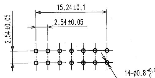
RECOMMENDED PC BOARD HOLE PATTERN
