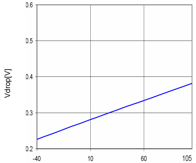
Fig.30 Minimum dropout Voltage1 (Vcc=6V、Io=1.0A)
