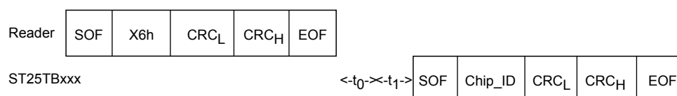
Figure 24. Slot_marker frame exchange between reader and ST25TB512-AT
