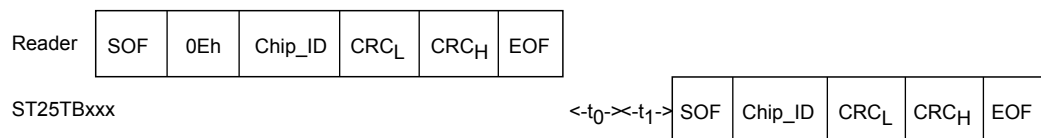
Figure 27. Select frame exchange between reader and ST25TB512-AT
