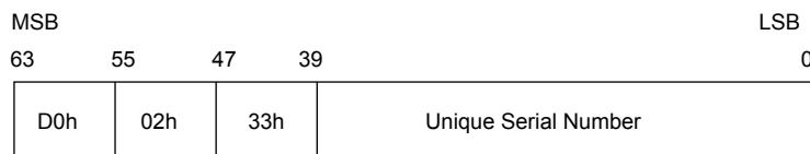
Figure 42. 64-bit unique identifier of the ST25TB512-AT
