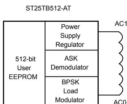
Figure 1. Logic diagram
