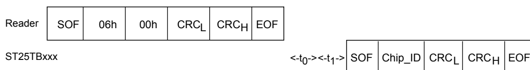
Figure 18. Initiate frame exchange between reader and ST25TB512-AT
