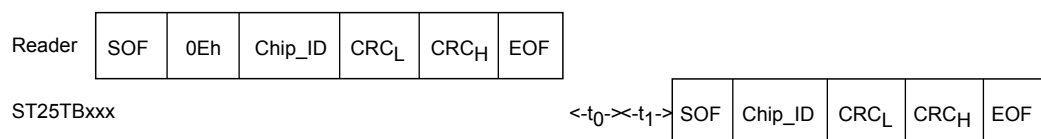
Figure 48. Select frame exchange between reader and ST25TB512-AT
