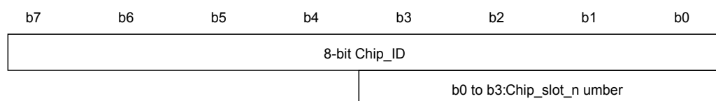
Figure 14. ST25TB512-AT Chip_ID description
