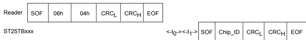
Figure 46. Pcall16 frame exchange between reader and ST25TB512-AT
