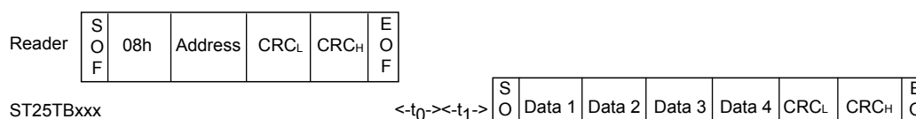
Figure 36. Read_block frame exchange between reader and ST25TB512-AT
