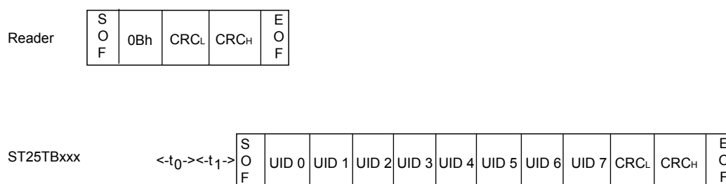
Figure 53. Get_UID frame exchange between reader and ST25TB512-AT
