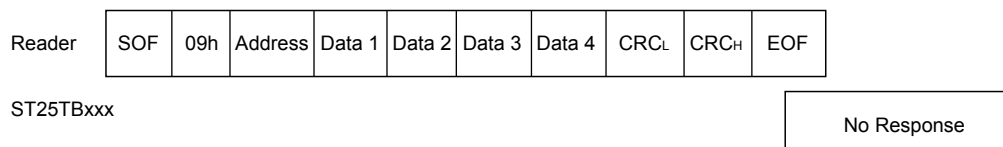
Figure 39. Write_block frame exchange between reader and ST25TB512-AT
