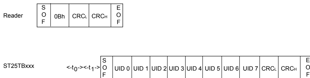
Figure 43. Get_UID frame exchange between reader and ST25TB512-AT
