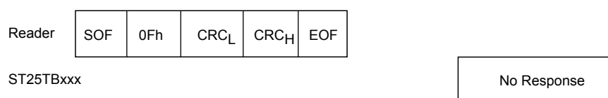
Figure 30. Completion frame exchange between reader and ST25TB512-AT
