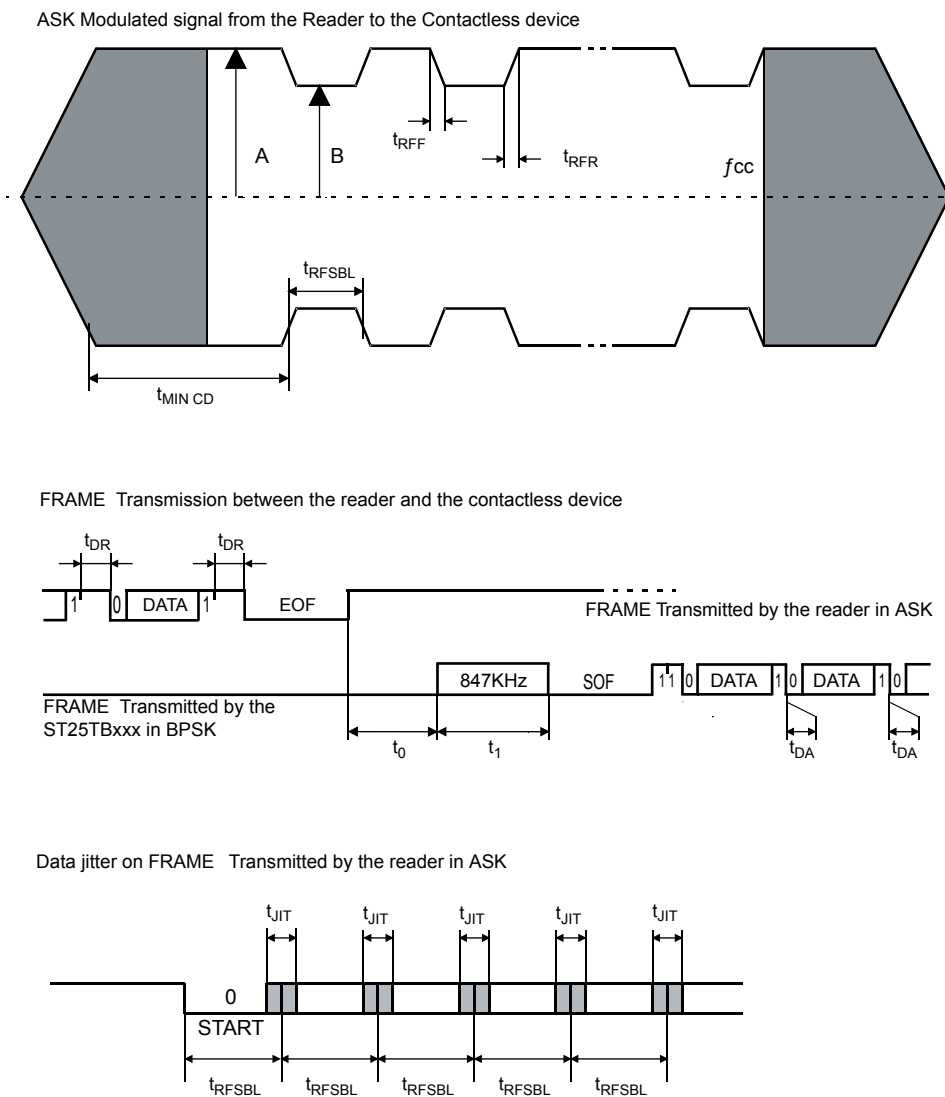
Figure 44. ST25TB512-AT synchronous timing, transmit and receive
