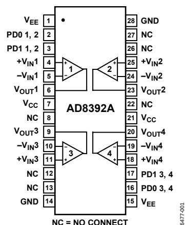
Figure 1. AD8392AARE, 28-Lead TSSOP/EP
