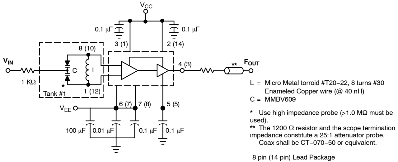
Tank Circuit Option #1, Varactor Diode
