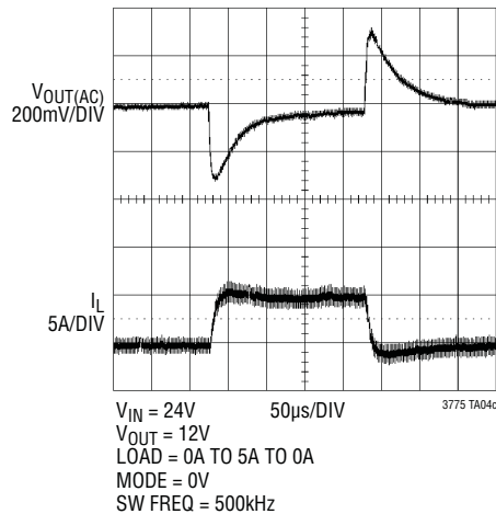
Load Step
