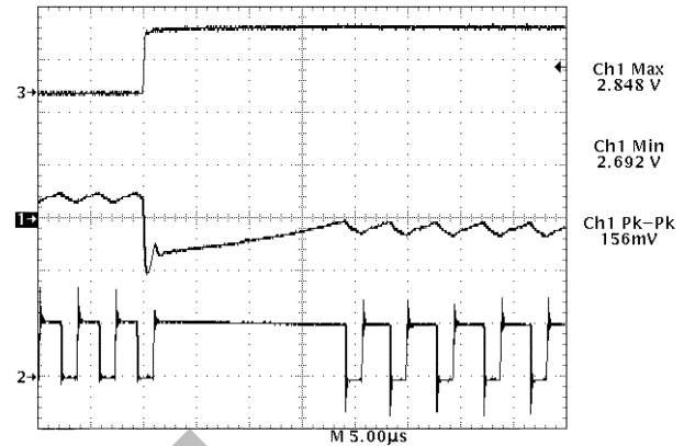
Figure 10. CS5157 Demonstration Board Response to 13 A Load Turn On (Output Set for 2.8 V). Upon Completing a Normal Off Time, The V^2 Control Loop Immediately Connects the Inductor to the Input Voltage, Providing 100% Duty Cycle. Regulation is Achieved in Less Than 20 \mu s
