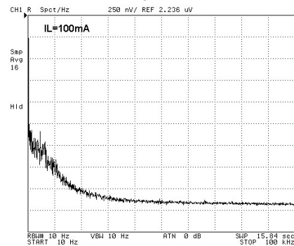
Output Noise
