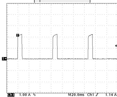
Short Circuit-Current
